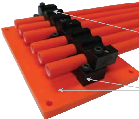
Mounting Bracket (secures each row of MicroDucts, includes 3 screws)
